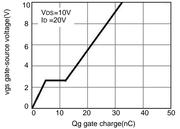
Fig.4 gate charge
