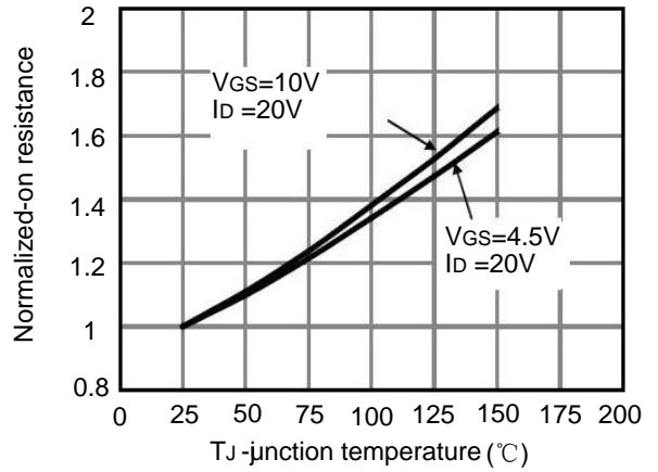
Fig.2 rdson-junction temperature
