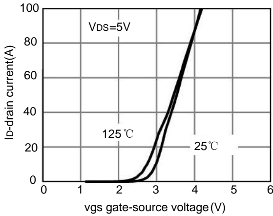
Fig.3 transfer characteristics
