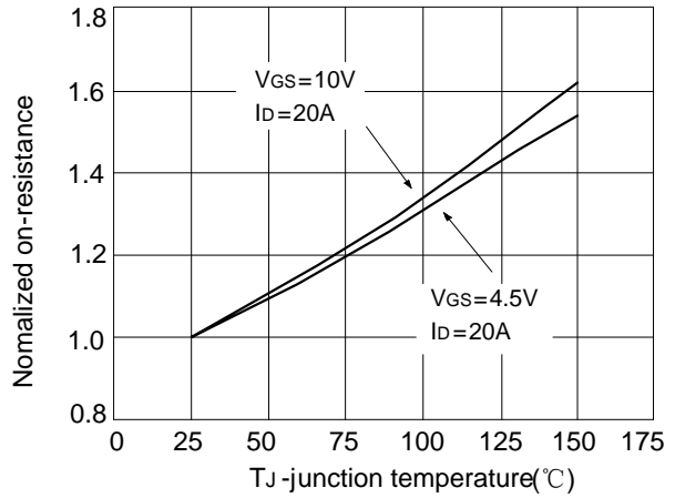
Fig.2 rdson-junction temperature
