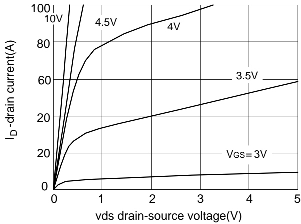
Fig.1 output characteristics
