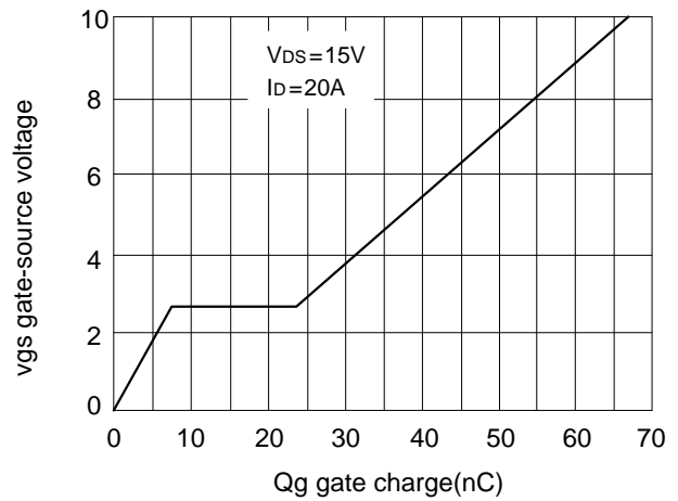
Fig.4 gate charge
