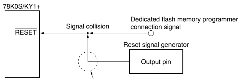
Figure 16-6. Signal Collision ( \overline{\text{RESET}} Pin)
