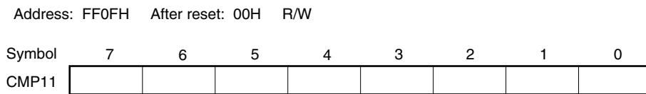
Figure 7-3. Format of 8-bit Timer H Compare Register 11 (CMP11)
