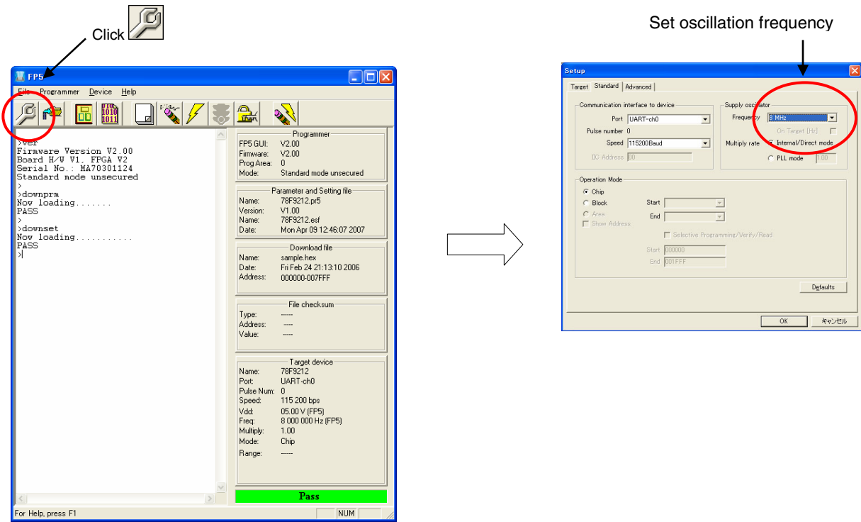
Figure 16-5. PG-FP5 GUI Software Setting Example
