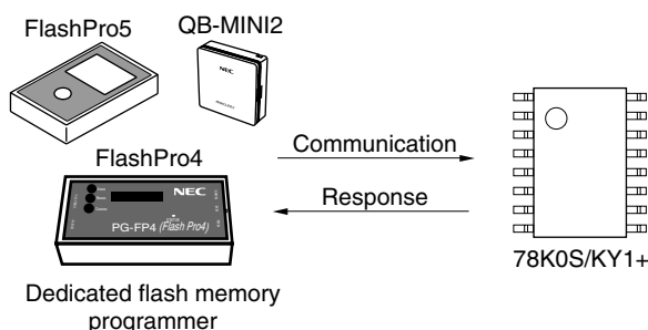
Figure 16-7. Communication Commands
