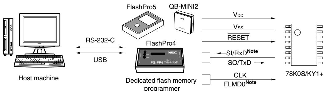
Figure 16-2. Environment for Writing Program to Flash Memory (FlashPro4/FlashPro5/QB-MINI2)
