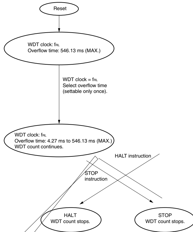
Figure 8-5. Status Transition Diagram When “Low-Speed Internal Oscillator Can Be Stopped by Software” Is Selected by Option Byte
