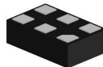
DFN1107-6L (Bottom view)
