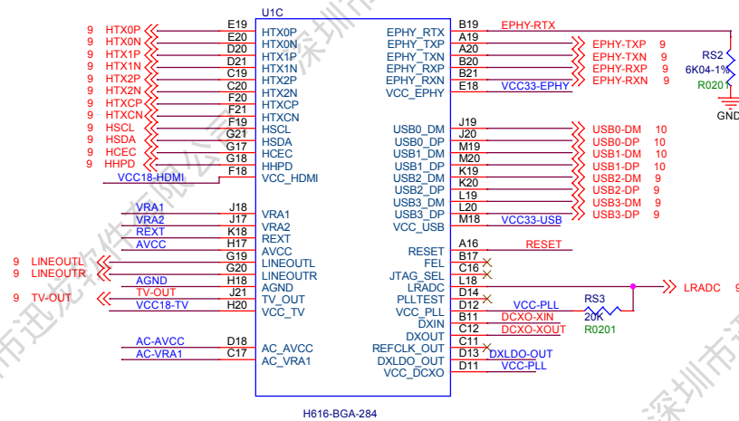
H616-BGA-284
