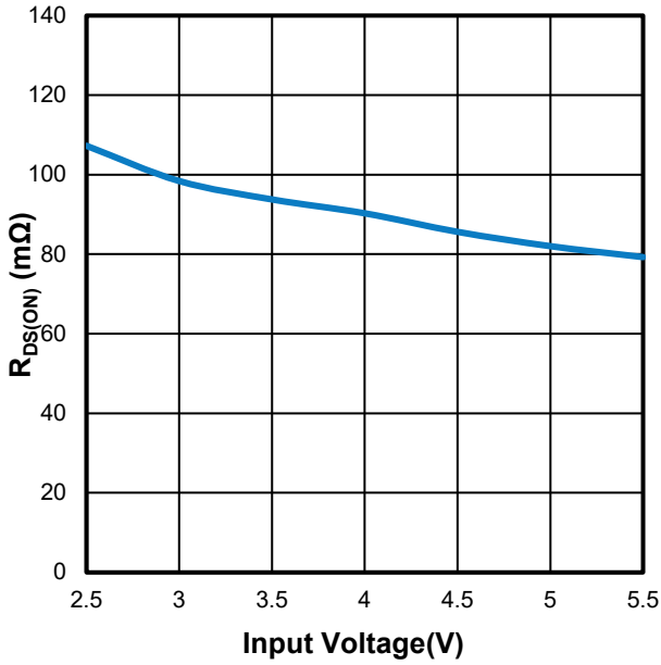
Switch On-Resistance vs. Input Voltage
