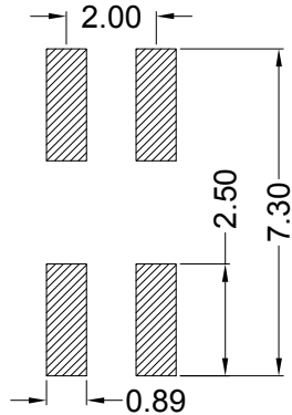
Recommended P. C. B LAYOUT General Tolerance \pm 0.05
