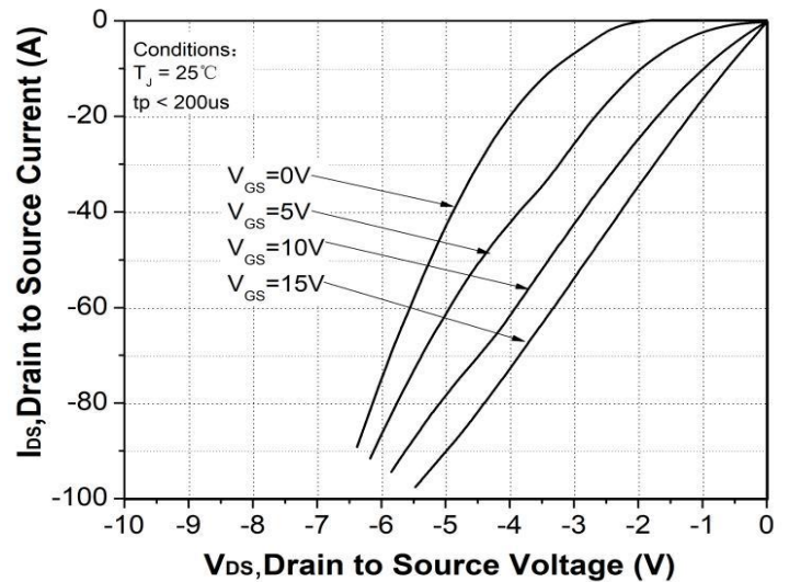
Figure 14. 3rd quadrant characteristic at T_J = 25^\circ\text{C}
