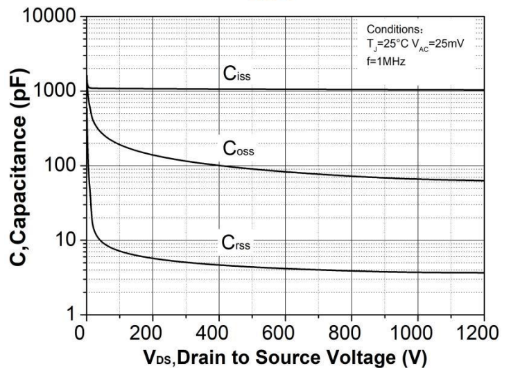
Figure 18. Capacitances vs. drain-source voltage (0 - 1200V)
