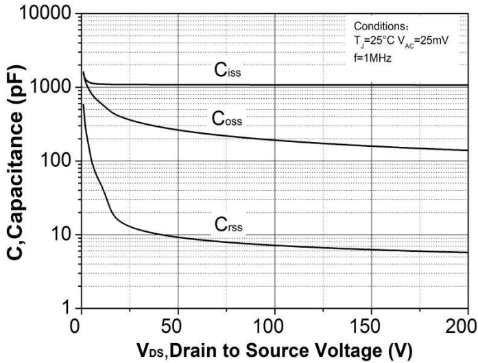
Figure 17. Capacitances vs. drain-source voltage (0 - 200V)
