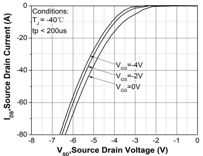
Figure 8. Body diode characteristic at T_J = -40^\circ\text{C}
