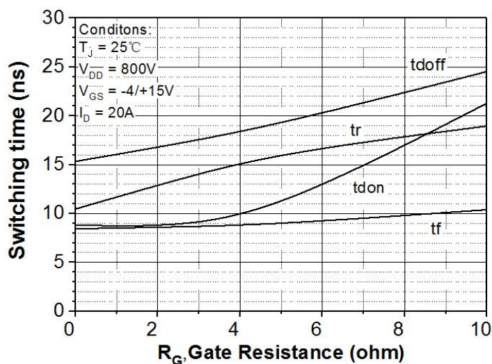
Figure 26. Switching times vs. R_G(\text{ext})
