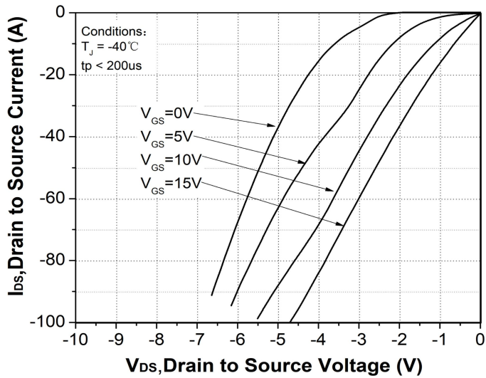
Figure 13. 3rd quadrant characteristic at T_J = -40^\circ\text{C}
