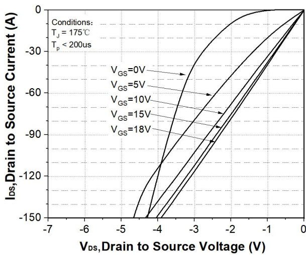
Figure 15. 3rd quadrant characteristic at T_J = 175\text{ }^\circ\text{C}
