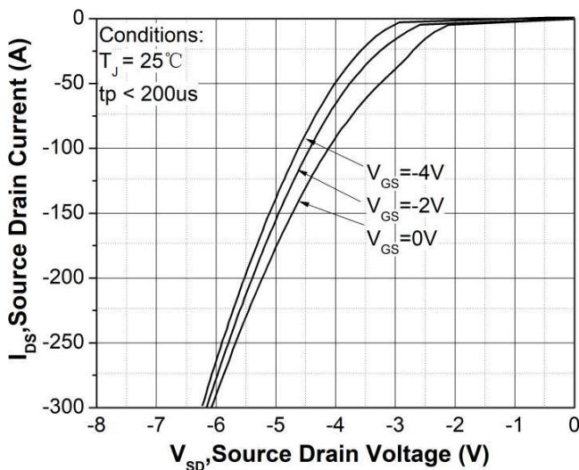
Figure 9. Body diode characteristic at T_J = 25^\circ\text{C}
