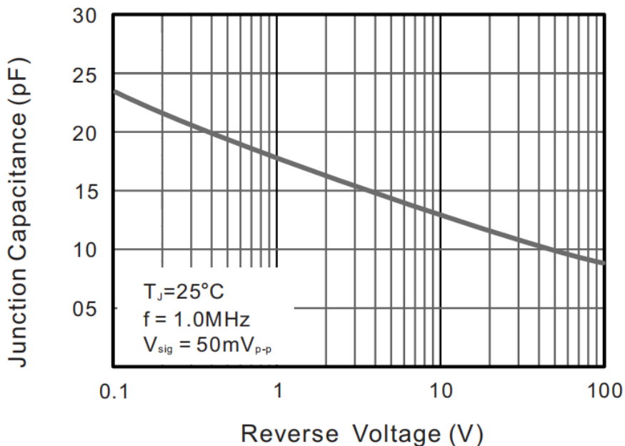
Fig.5 Typical Junction Capacitance
