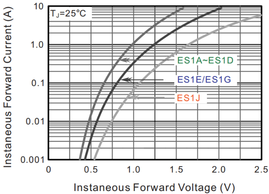
Fig.4 Typical Forward Characteristics
