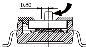
[推钮行程]
