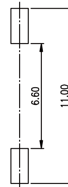
RECOMMENDED P.C.B. LAYOUT (TOP VIEW)
