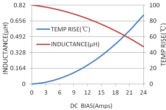
FSA0630-R82MT
