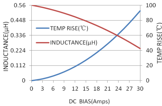
FSA0630-R82MT
