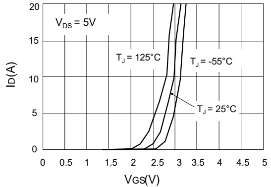
Fig.2 Transfer characteristics
