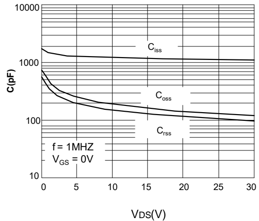
Fig.6 Capacitance characteristics
