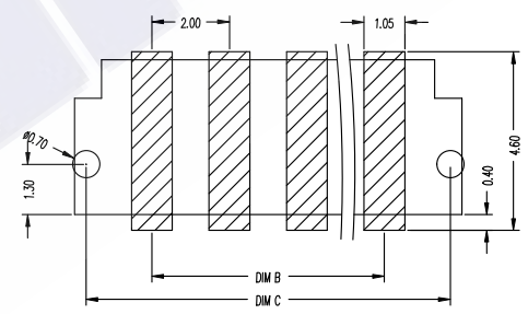
RECOMMENDED PCB LAYOUT TOL: (±0.05)
