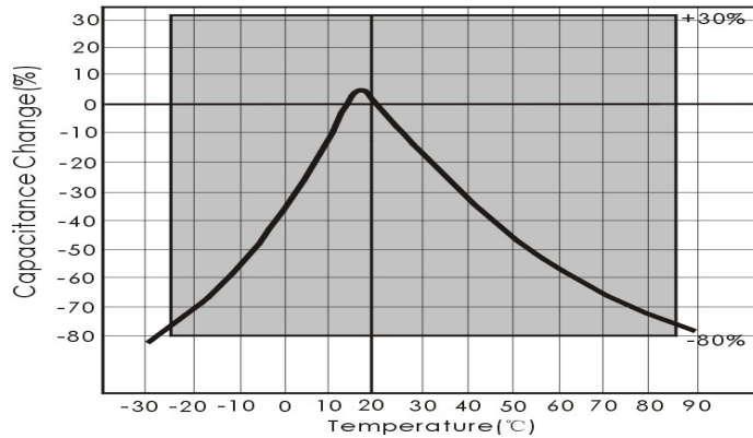
Char:F (Y5V)
