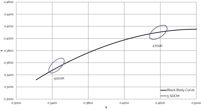
Figure 13: Graph of Test Bins in xy Color Space
