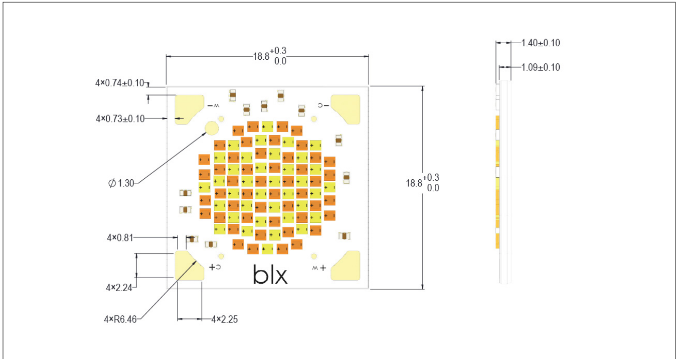
Figure 12: Drawing for Vesta Series Tunable White 13mm Array
