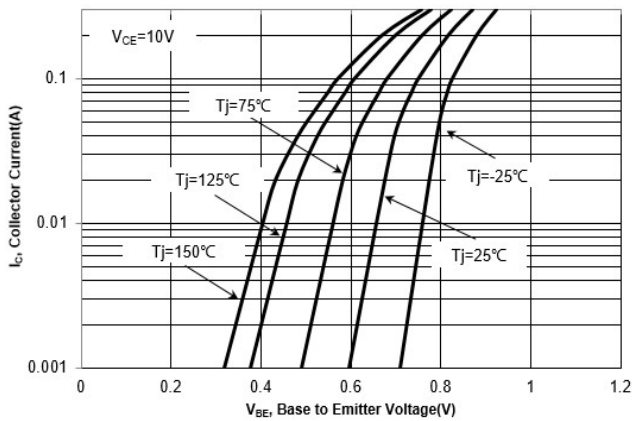
Fig. 3 Collector Current vs. Base to Emitter Voltage
