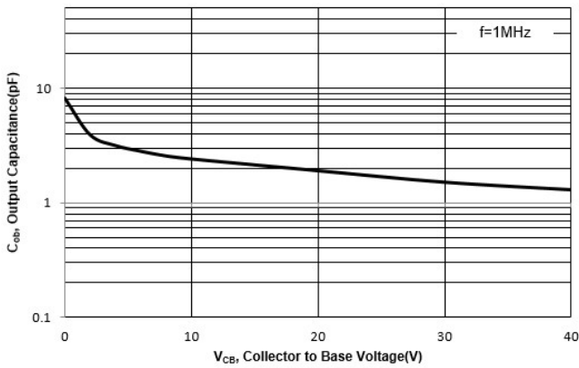
Fig. 7 Output Capacitance
